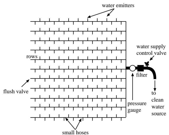
Figure 24. Diagram of trickle irrigation system set up to water small garden area. Plants are set by water emitters.
